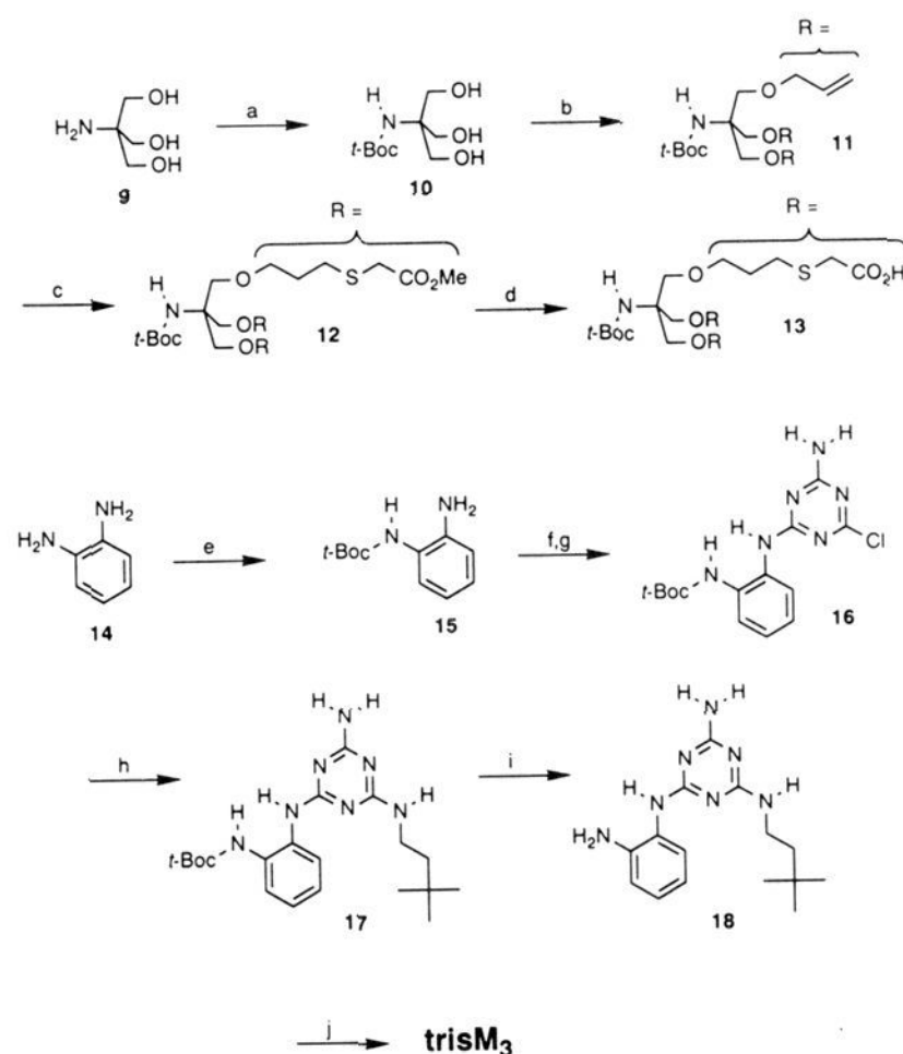
Scheme IV. Synthesis of trisM 3 a
