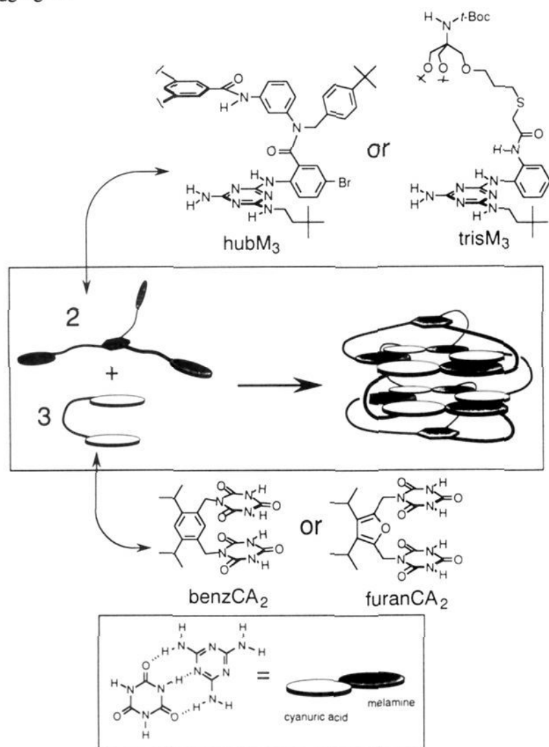
Scheme II. Self-Assembly of 2 equiv of hubM 3 or trisM 3 with 3 equiv of benzCA 2 or furanCA 2 To Give a 2 + 3 Supramolecular Aggregate
