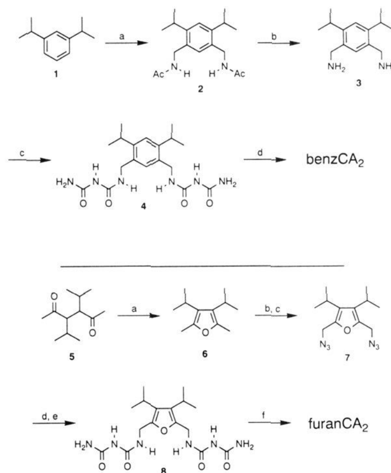
Scheme III. Synthesis of benzCA 2 a and furanCA 2 b
